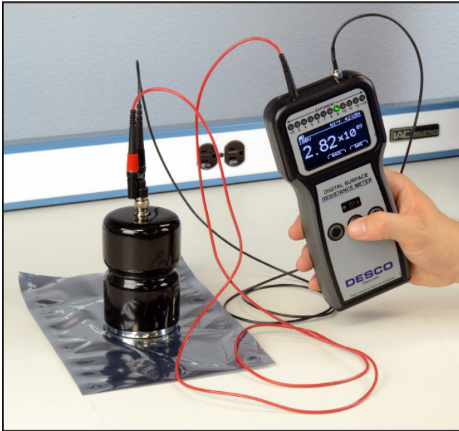
Figure 3. Using the Concentric Ring Probe with the Desco Digital Surface Resistance Meter
